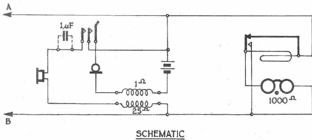
MAGNETO TELEPHONE (TABLE TYPE).
